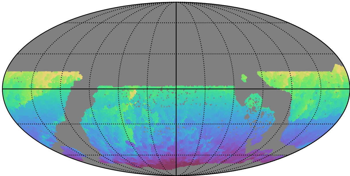
too_elab_r8_d2_ugrizy_v3.4_10yrs WFD all bands: Min HA
