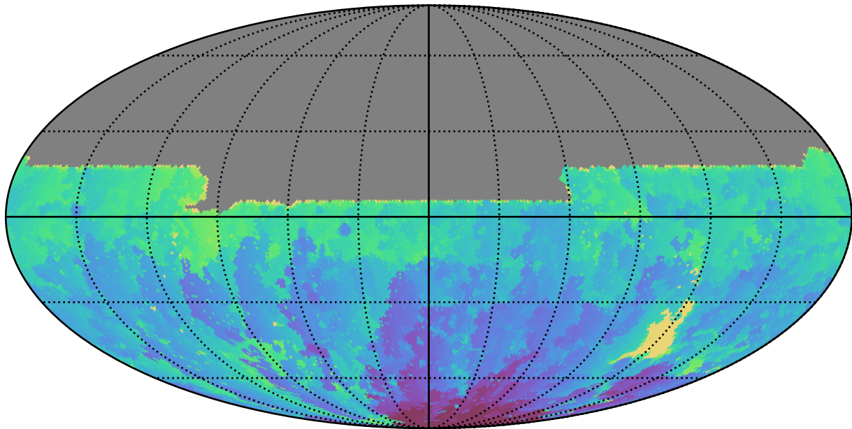
too_elab_r8_d2_ugrizy_v3.4_10yrs All sky u band: Min HA
