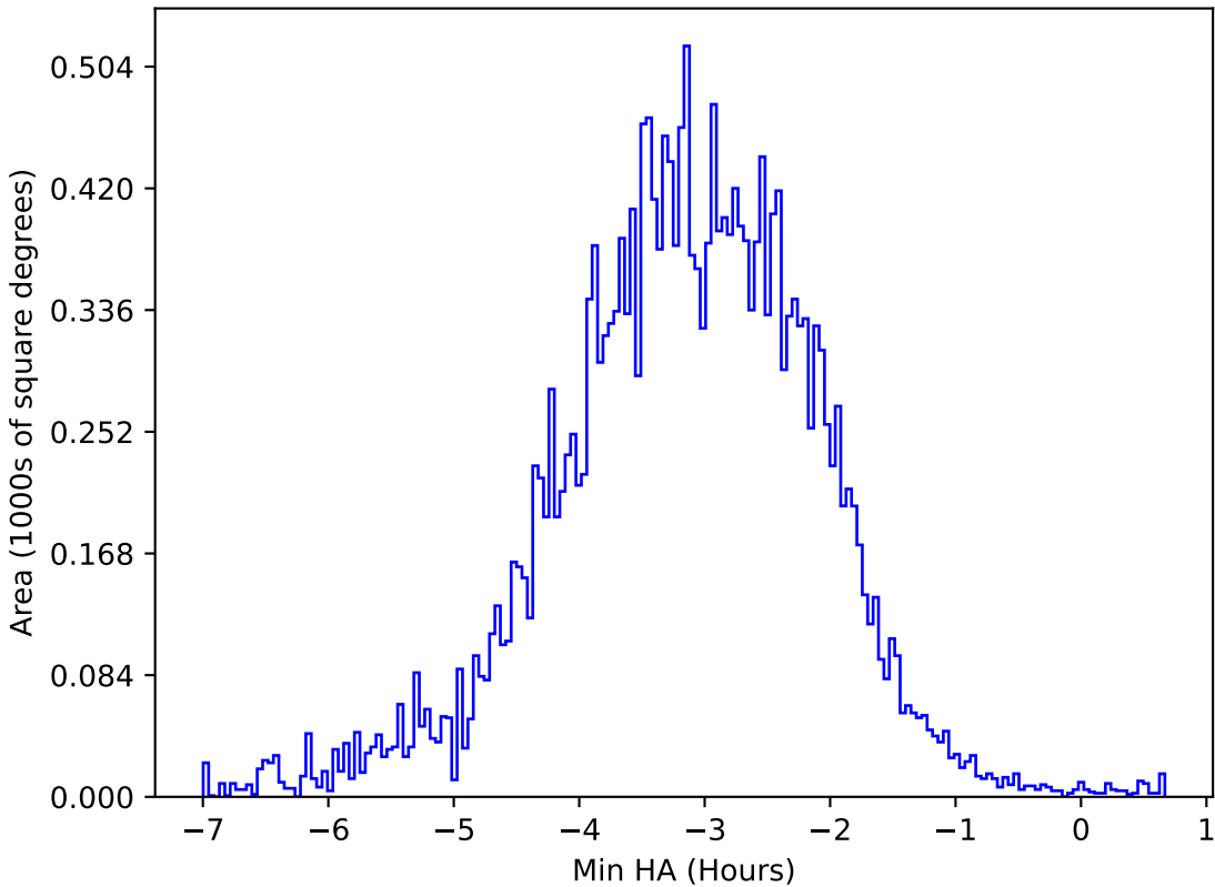
too_elab_r8_d2_ugrizy_v3.4_10yrs All sky u band: Min HA
