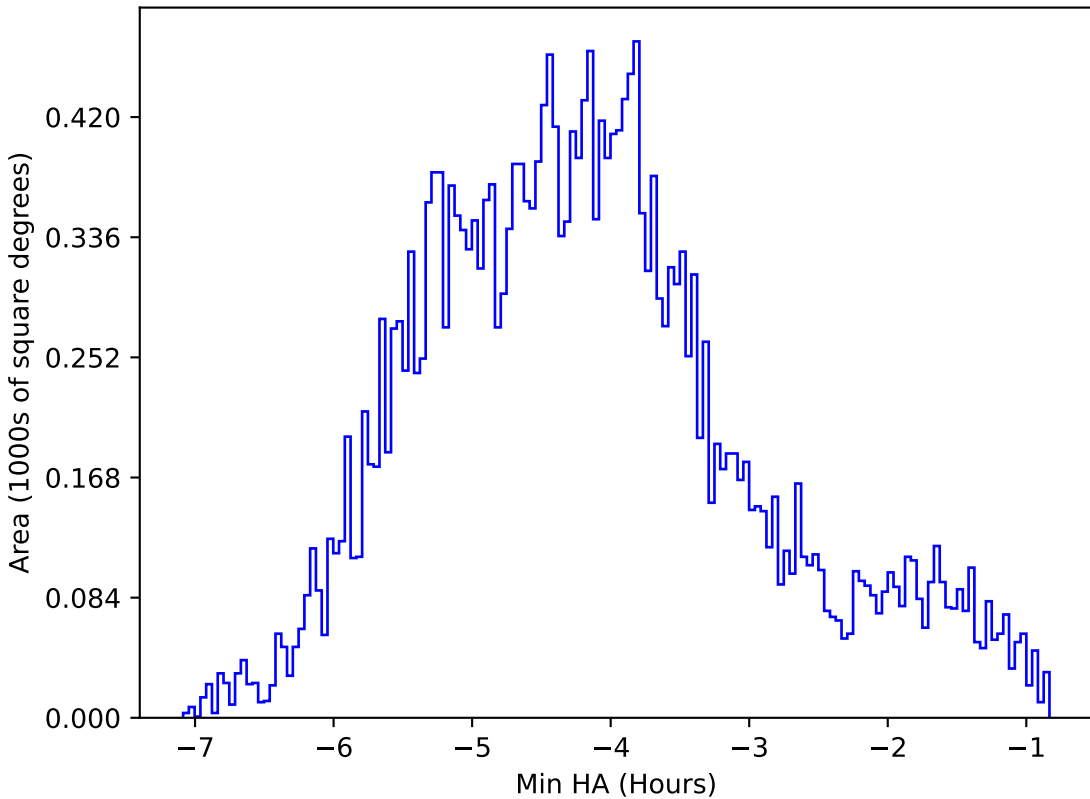
too_elab_r8_d2_ugrizy_v3.4_10yrs All sky r band: Min HA
