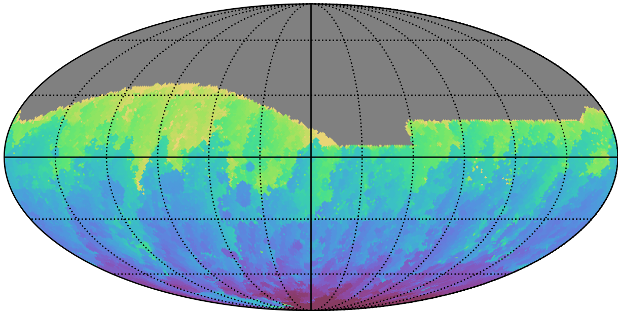
too_elab_r8_d2_ugrizy_v3.4_10yrs All sky g band: Min HA
