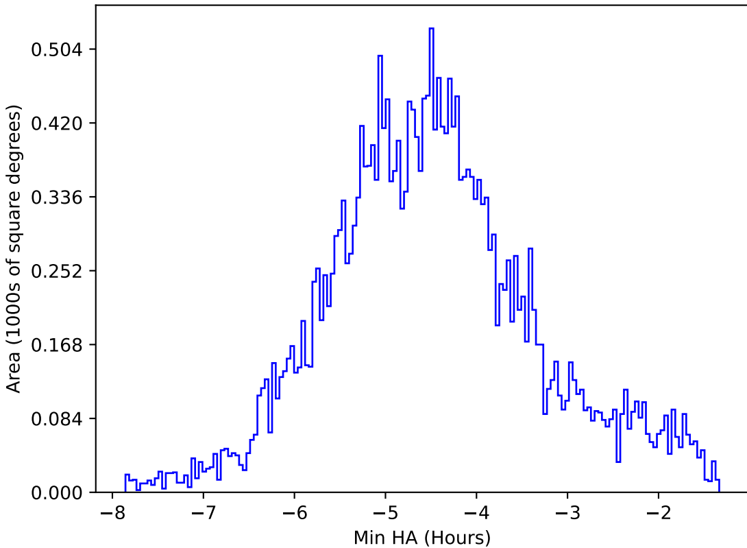
too_elab_r8_d2_ugrizy_v3.4_10yrs All sky all bands: Min HA
