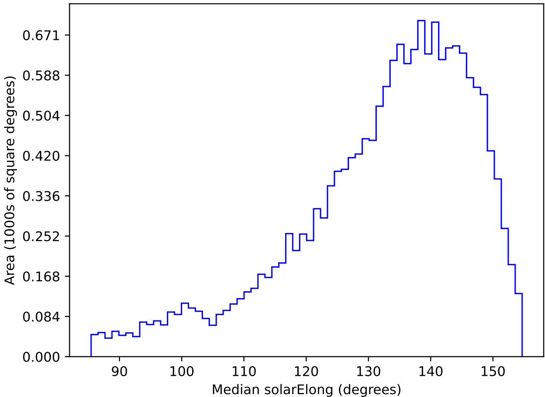
too_elab_r8_d2_ugrizy_v3.4_10yrs WFD u band: Median solarElong
