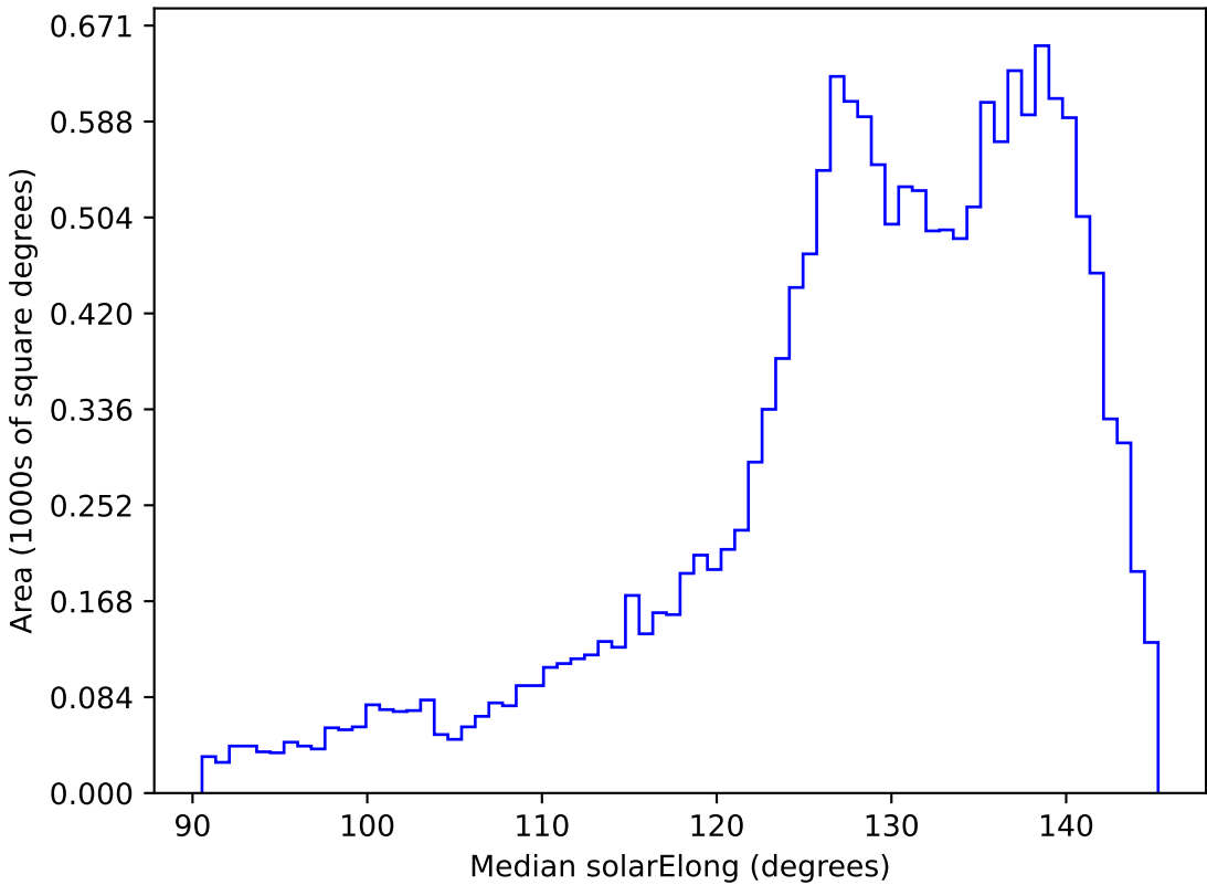
too_elab_r8_d2_ugrizy_v3.4_10yrs WFD i band: Median solarElong
