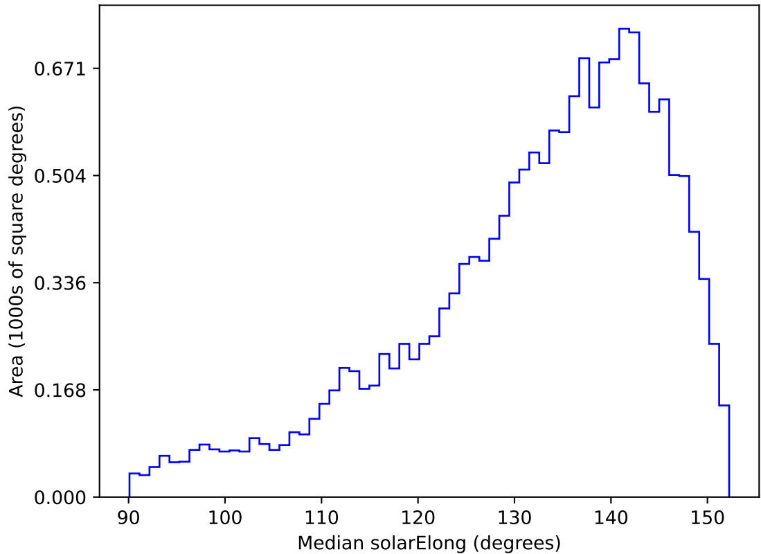
too_elab_r8_d2_ugrizy_v3.4_10yrs WFD g band: Median solarElong
