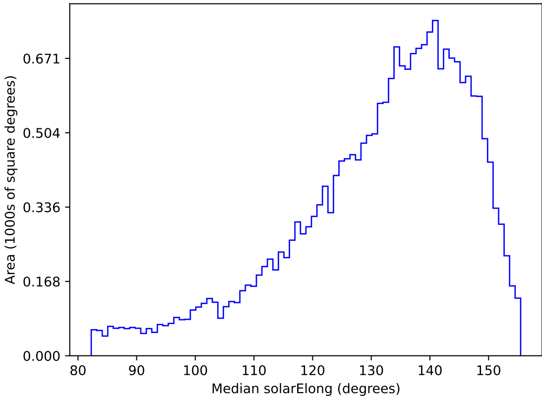
too_elab_r8_d2_ugrizy_v3.4_10yrs All sky u band: Median solarElong
