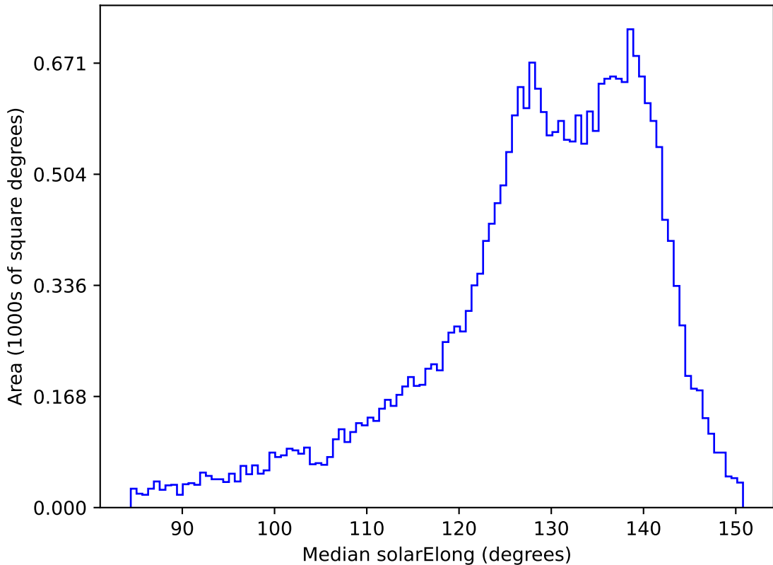
too_elab_r8_d2_ugrizy_v3.4_10yrs All sky i band: Median solarElong
