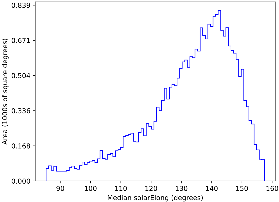
too_elab_r8_d2_ugrizy_v3.4_10yrs All sky g band: Median solarElong
