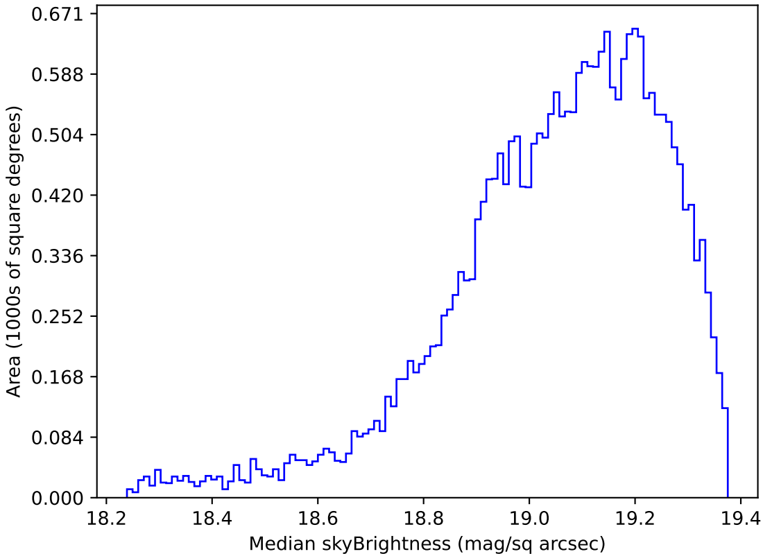
too_elab_r8_d2_ugrizy_v3.4_10yrs Yr 1 z band: Median skyBrightness
