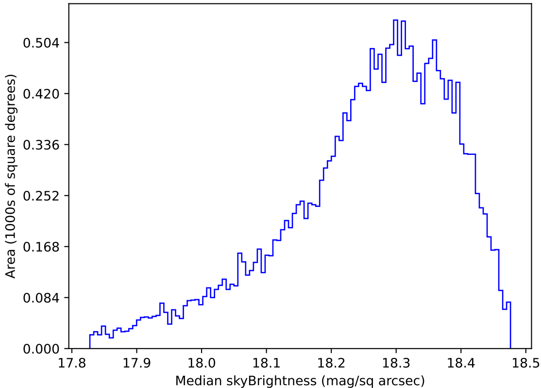
too_elab_r8_d2_ugrizy_v3.4_10yrs Yr 1 y band: Median skyBrightness
