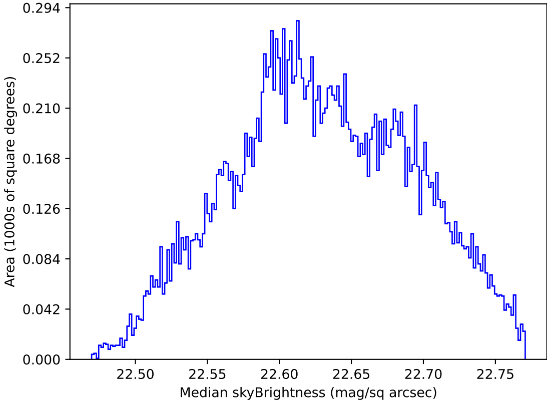
too_elab_r8_d2_ugrizy_v3.4_10yrs Yr 1 u band: Median skyBrightness
