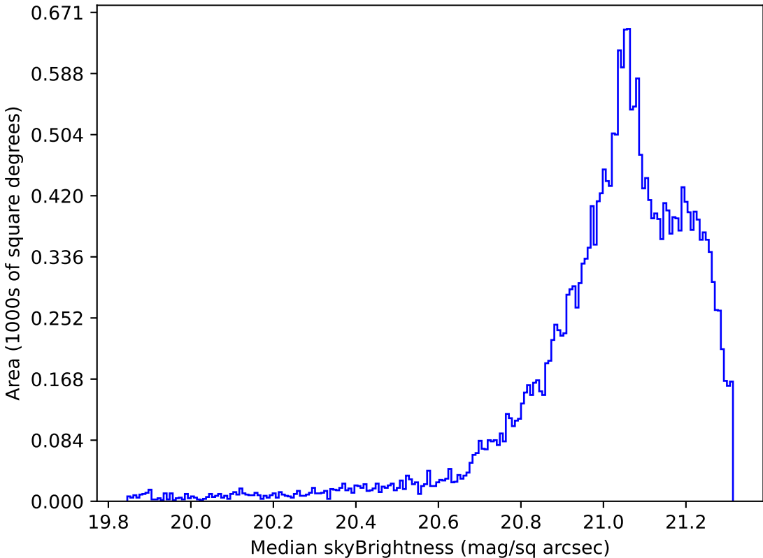
too_elab_r8_d2_ugrizy_v3.4_10yrs Yr 1 r band: Median skyBrightness
