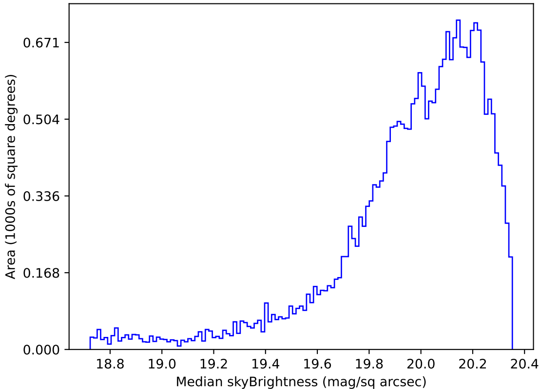
too_elab_r8_d2_ugrizy_v3.4_10yrs Yr 1 i band: Median skyBrightness
