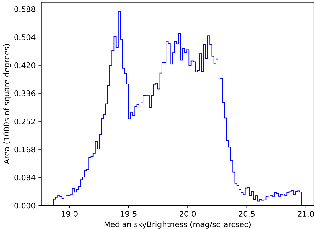
too_elab_r8_d2_ugrizy_v3.4_10yrs Yr 1 all bands: Median skyBrightness
