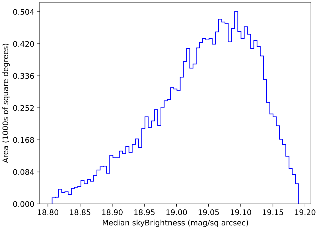
too_elab_r8_d2_ugrizy_v3.4_10yrs WFD z band: Median skyBrightness
