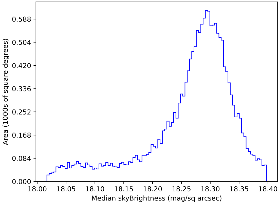
too_elab_r8_d2_ugrizy_v3.4_10yrs WFD y band: Median skyBrightness
