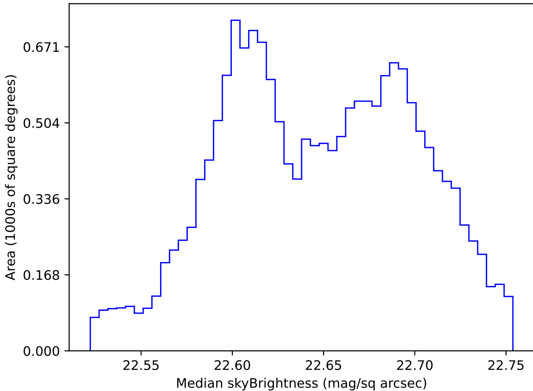
too_elab_r8_d2_ugrizy_v3.4_10yrs WFD u band: Median skyBrightness
