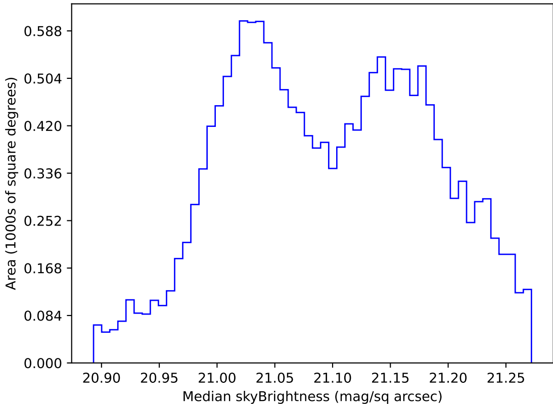
too_elab_r8_d2_ugrizy_v3.4_10yrs WFD r band: Median skyBrightness
