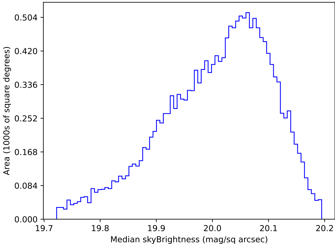
too_elab_r8_d2_ugrizy_v3.4_10yrs WFD i band: Median skyBrightness
