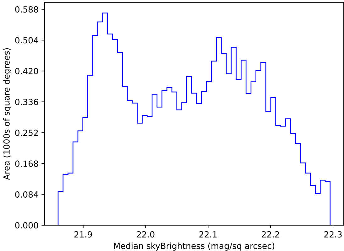
too_elab_r8_d2_ugrizy_v3.4_10yrs WFD g band: Median skyBrightness
