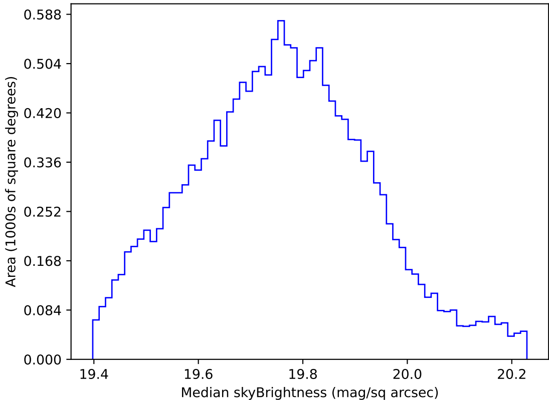
too_elab_r8_d2_ugrizy_v3.4_10yrs WFD all bands: Median skyBrightness
