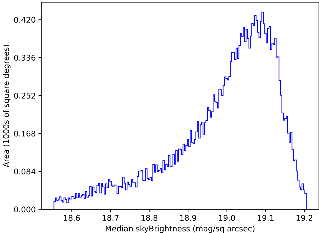
too_elab_r8_d2_ugrizy_v3.4_10yrs All sky z band: Median skyBrightness
