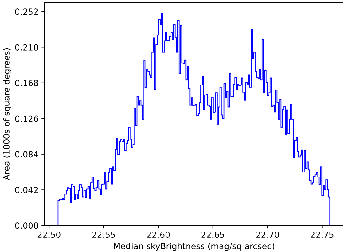
too_elab_r8_d2_ugrizy_v3.4_10yrs All sky u band: Median skyBrightness
