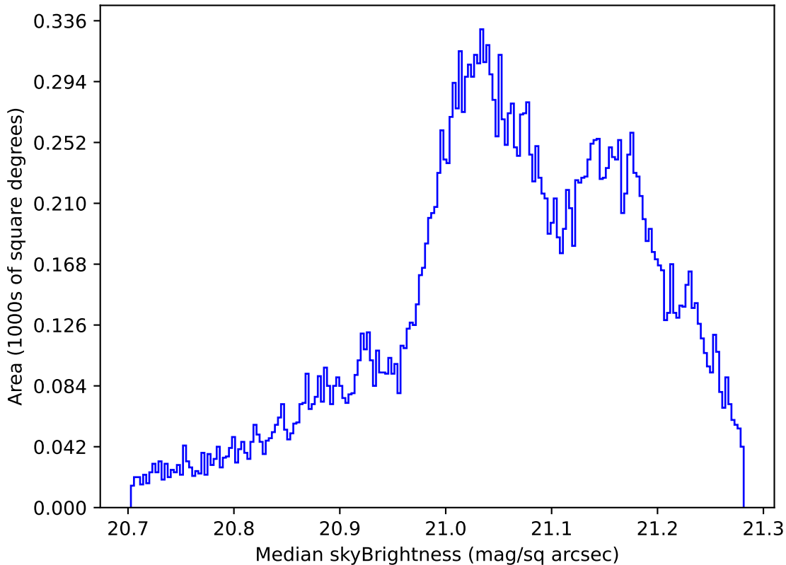
too_elab_r8_d2_ugrizy_v3.4_10yrs All sky r band: Median skyBrightness
