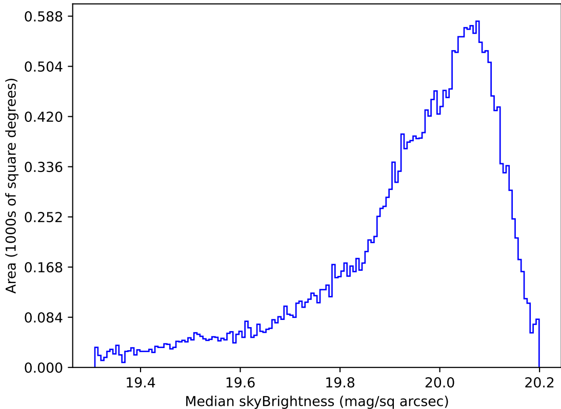
too_elab_r8_d2_ugrizy_v3.4_10yrs All sky i band: Median skyBrightness
