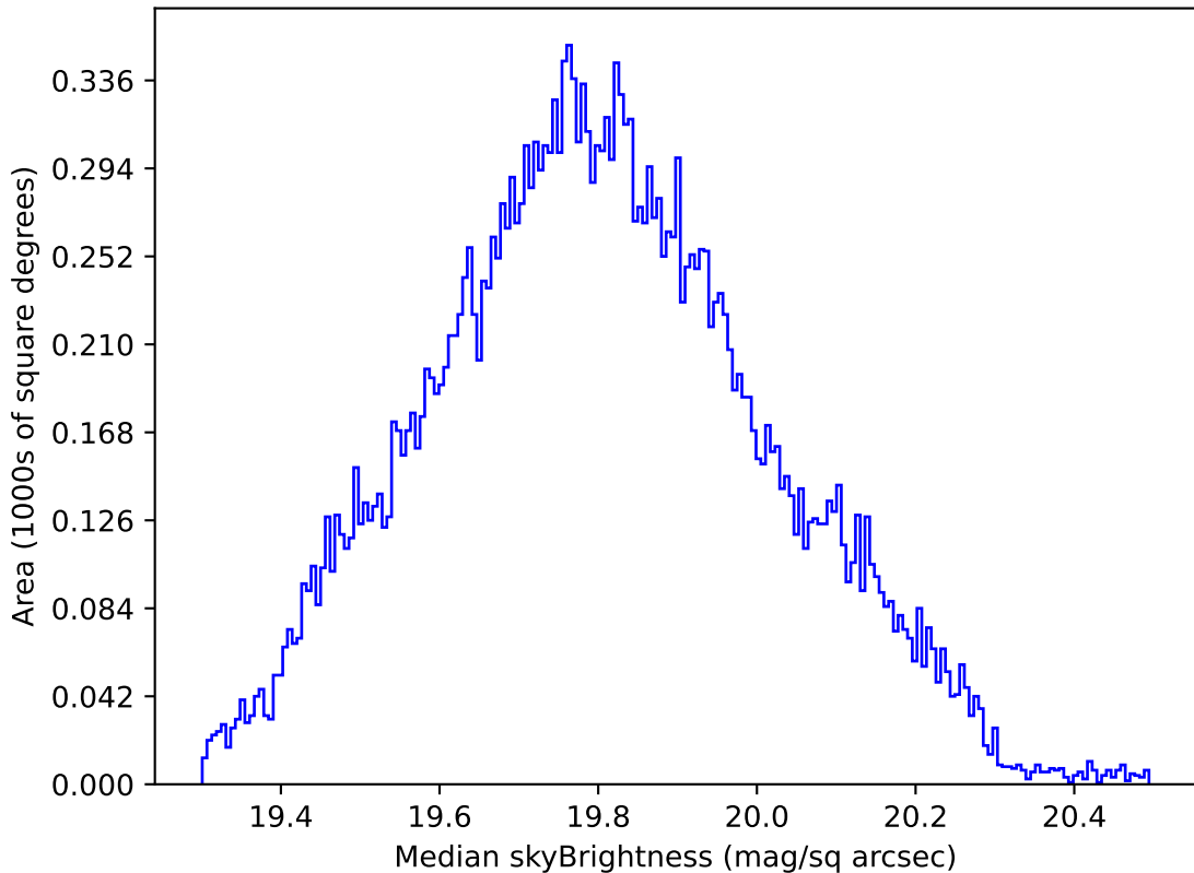
too_elab_r8_d2_ugrizy_v3.4_10yrs All sky all bands: Median skyBrightness
