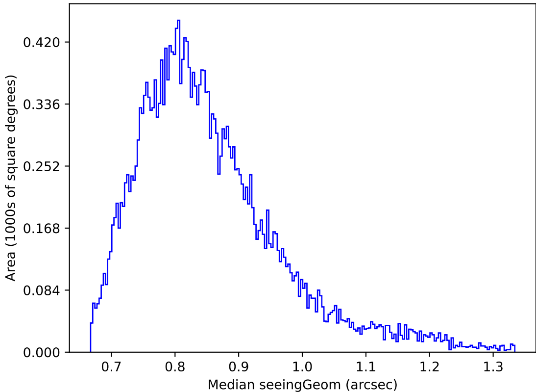
too_elab_r8_d2_ugrizy_v3.4_10yrs Yr 1 z band: Median seeingGeom
