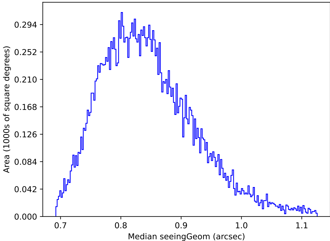
too_elab_r8_d2_ugrizy_v3.4_10yrs Yr 1 y band: Median seeingGeom
