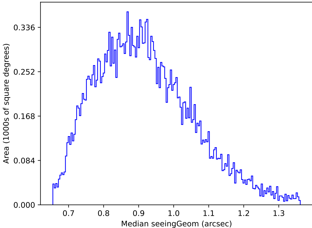
too_elab_r8_d2_ugrizy_v3.4_10yrs Yr 1 g band: Median seeingGeom
