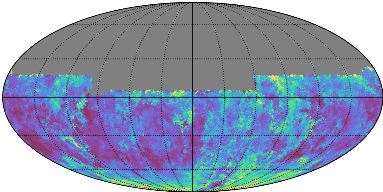
too_elab_r8_d2_ugrizy_v3.4_10yrs Yr 1 y band: Median seeingEff
