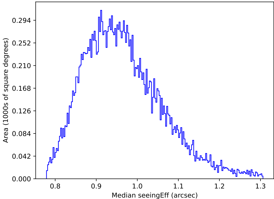
too_elab_r8_d2_ugrizy_v3.4_10yrs Yr 1 y band: Median seeingEff
