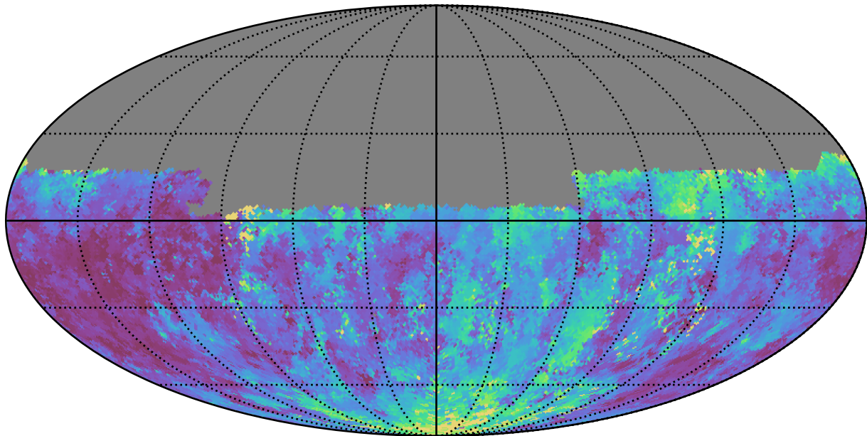
too_elab_r8_d2_ugrizy_v3.4_10yrs Yr 1 u band: Median seeingEff
