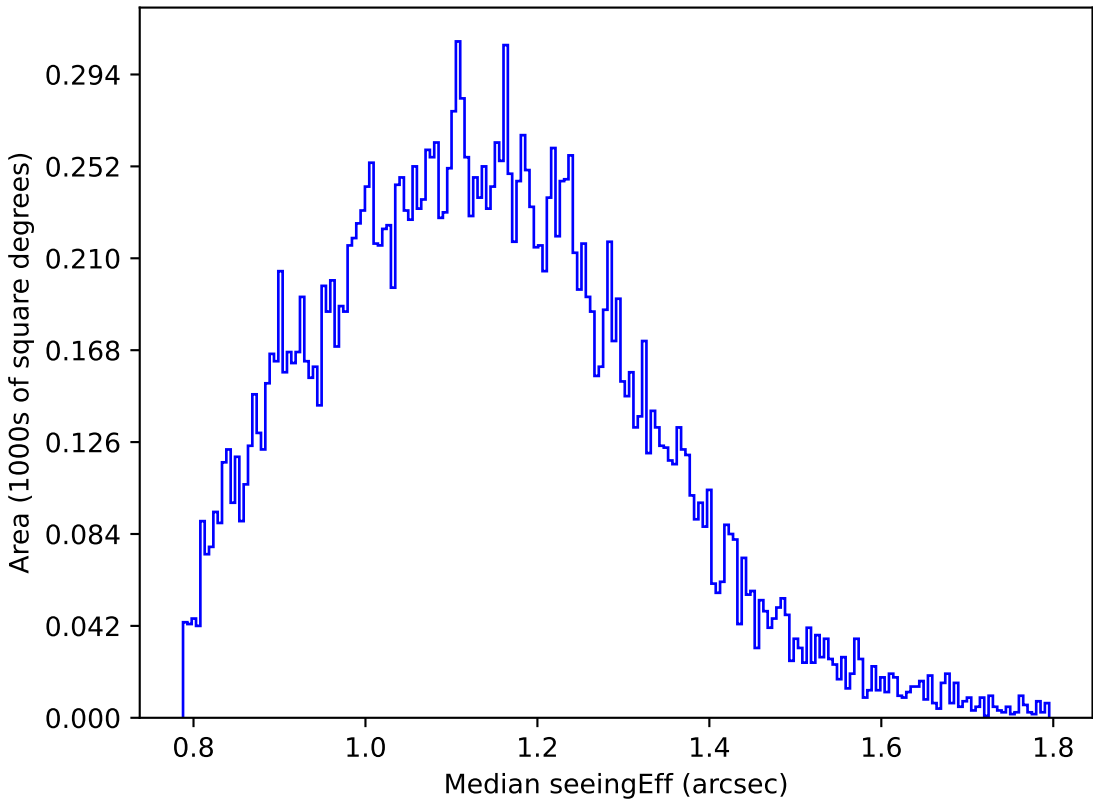
too_elab_r8_d2_ugrizy_v3.4_10yrs Yr 1 u band: Median seeingEff
