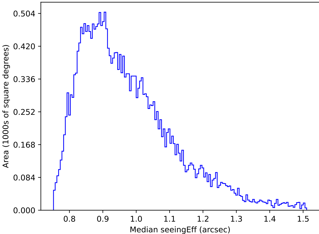
too_elab_r8_d2_ugrizy_v3.4_10yrs Yr 1 r band: Median seeingEff
