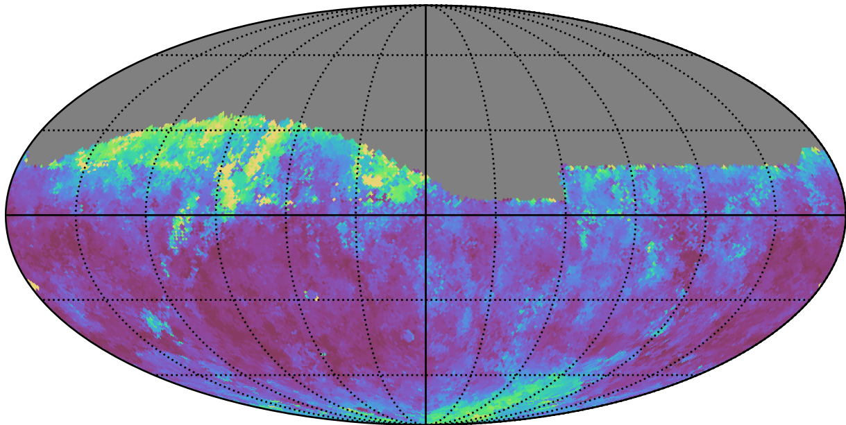
too_elab_r8_d2_ugrizy_v3.4_10yrs Yr 1 i band: Median seeingEff
