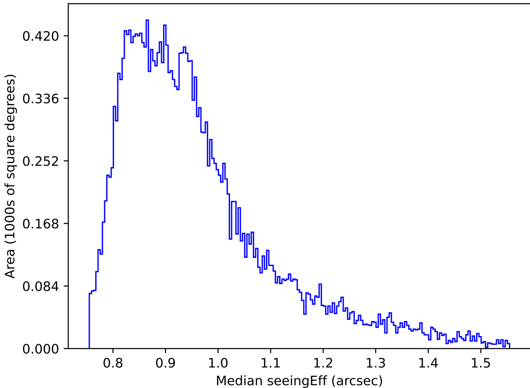
too_elab_r8_d2_ugrizy_v3.4_10yrs Yr 1 i band: Median seeingEff
