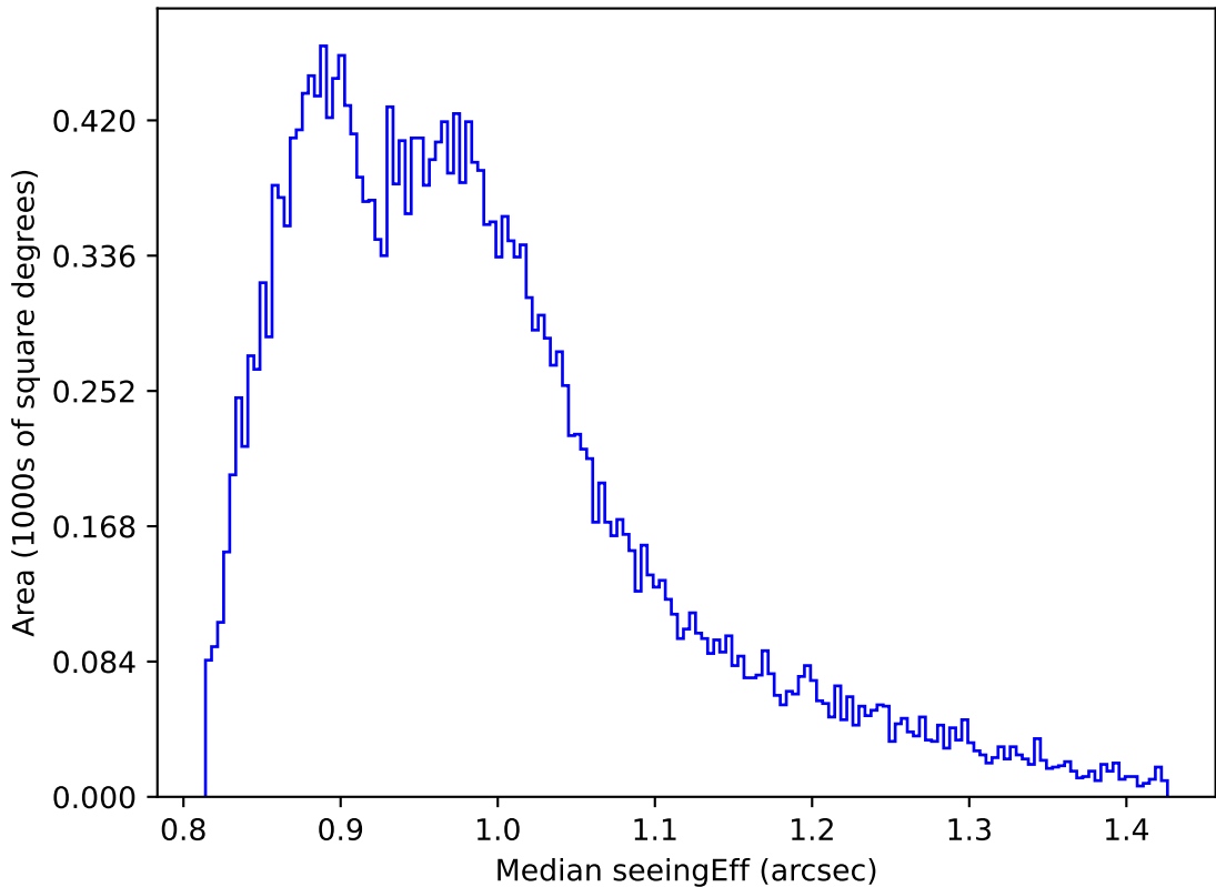
too_elab_r8_d2_ugrizy_v3.4_10yrs Yr 1 all bands: Median seeingEff
