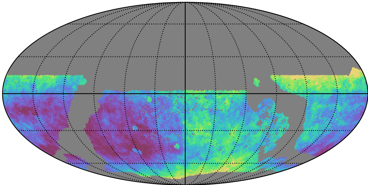
too_elab_r8_d2_ugrizy_v3.4_10yrs WFD z band: Median seeingEff
