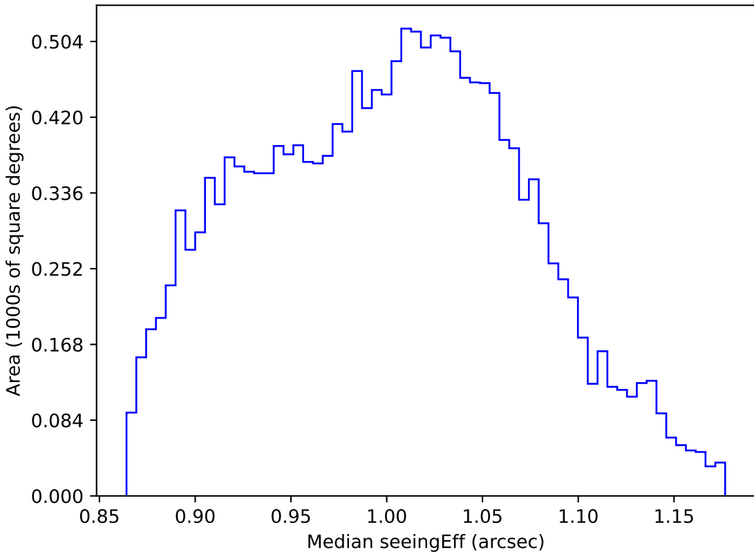
too_elab_r8_d2_ugrizy_v3.4_10yrs WFD z band: Median seeingEff
