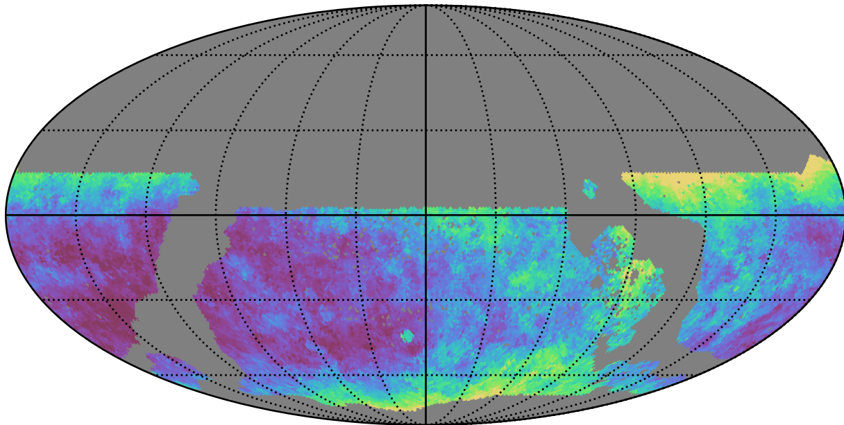
too_elab_r8_d2_ugrizy_v3.4_10yrs WFD y band: Median seeingEff
