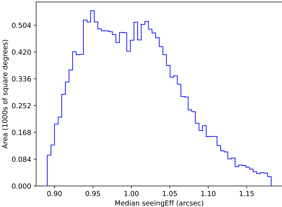
too_elab_r8_d2_ugrizy_v3.4_10yrs WFD y band: Median seeingEff
