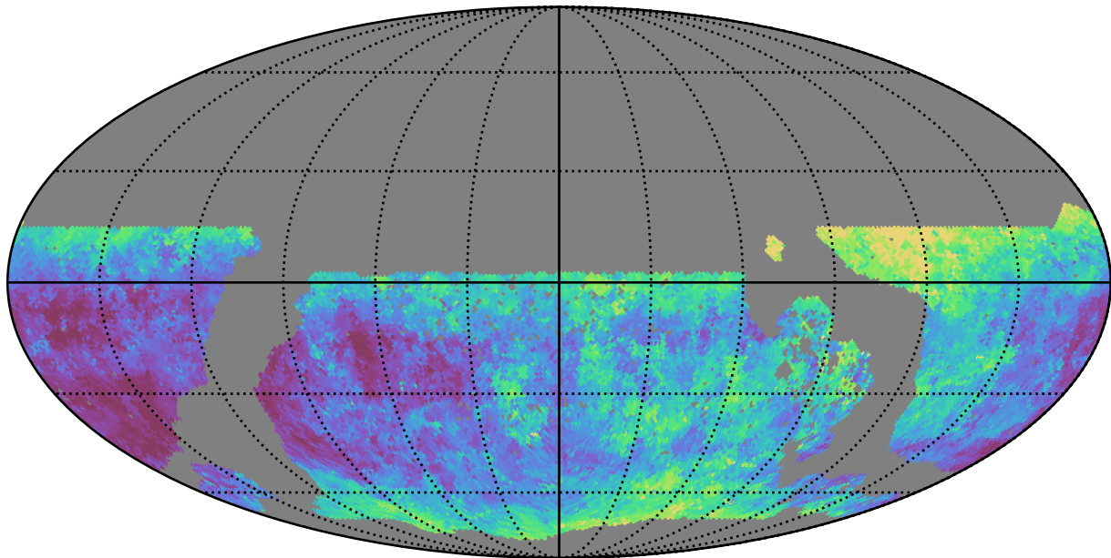
too_elab_r8_d2_ugrizy_v3.4_10yrs WFD u band: Median seeingEff
