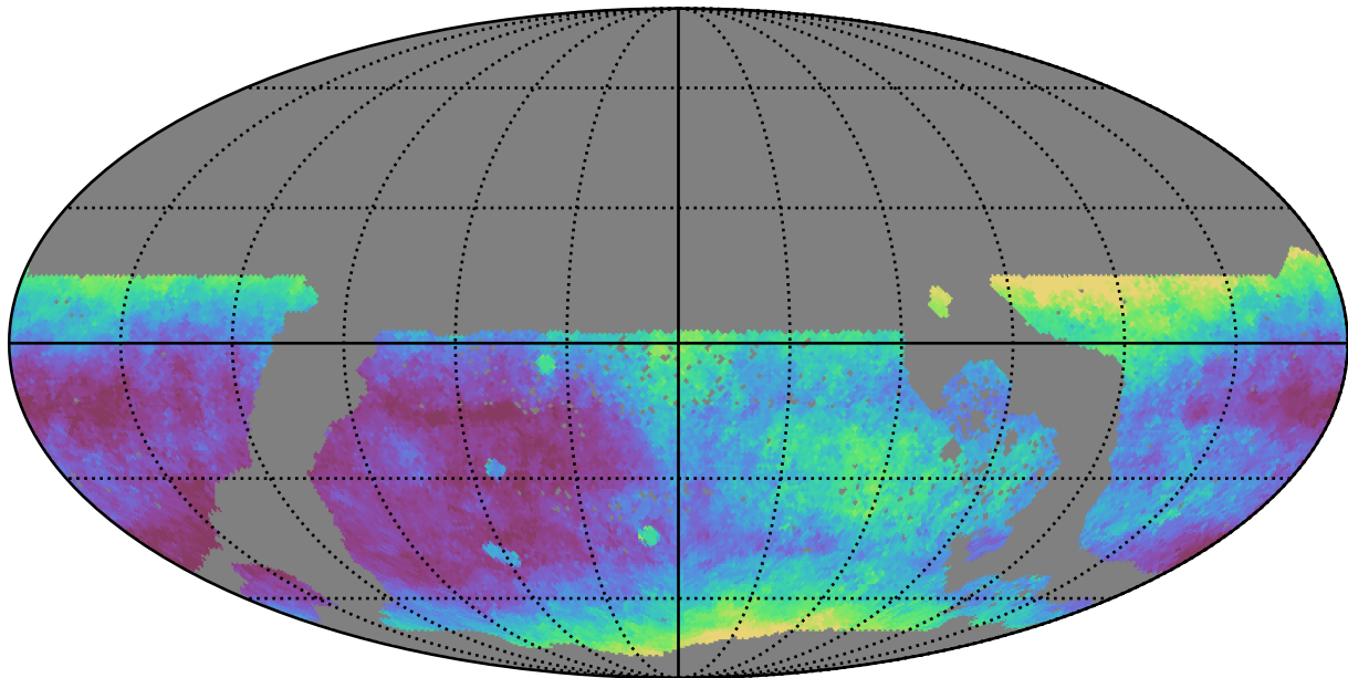
too_elab_r8_d2_ugrizy_v3.4_10yrs WFD r band: Median seeingEff
