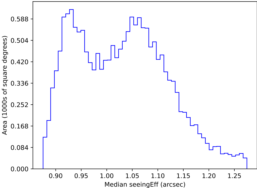
too_elab_r8_d2_ugrizy_v3.4_10yrs WFD r band: Median seeingEff
