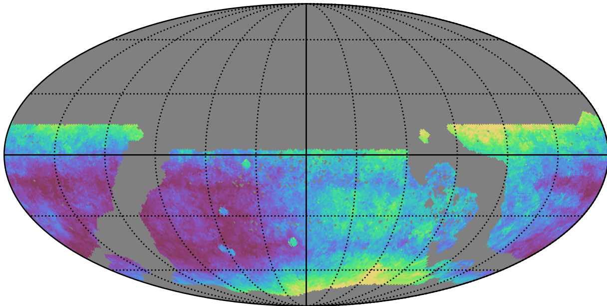
too_elab_r8_d2_ugrizy_v3.4_10yrs WFD i band: Median seeingEff
