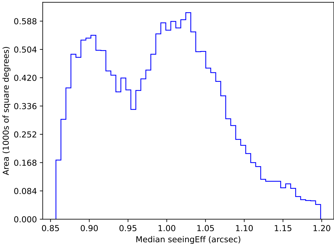
too_elab_r8_d2_ugrizy_v3.4_10yrs WFD i band: Median seeingEff
